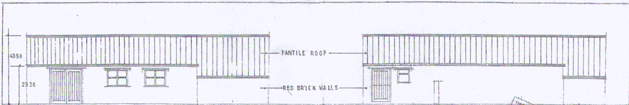
BUILDING 1 FRONT ELEVATION ↔ SOUTH EAST (SUBJECT OF APPLICATION)
